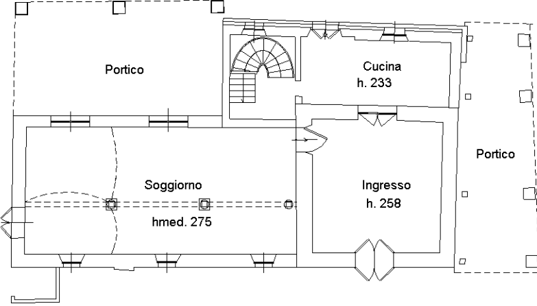
PIANO TERRA
